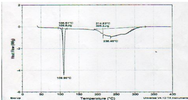
Fig.4: DSC Curve of Pure Drug
