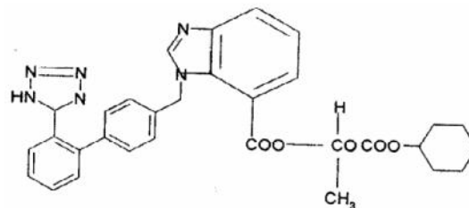
Fig 1: Structure of Candesartan Cilexetil
