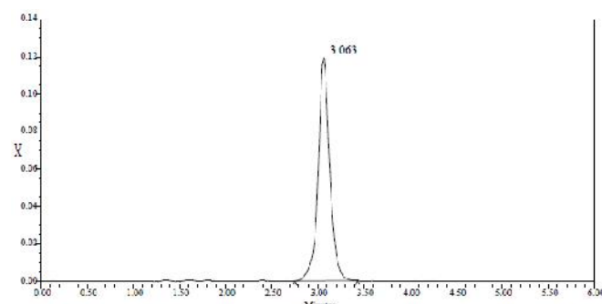
Fig. 4: The chromatogram of acid degraded sample
