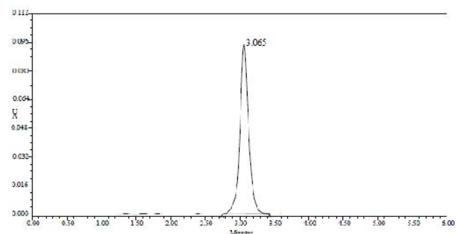
Fig. 6: The chromatogram of thermal degraded sample
